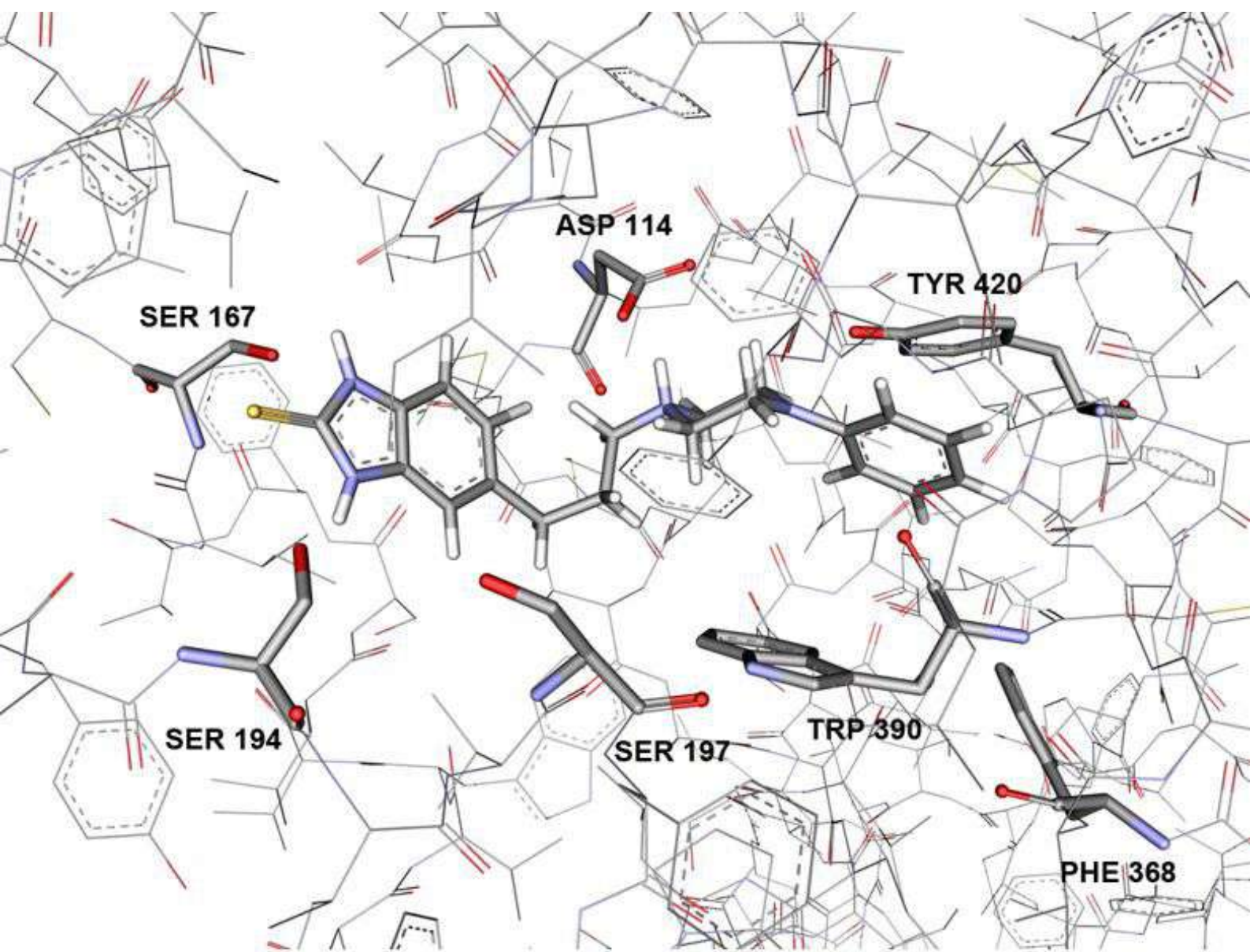
Docking results of ligand 10. Only key amino acid residues are marked.
