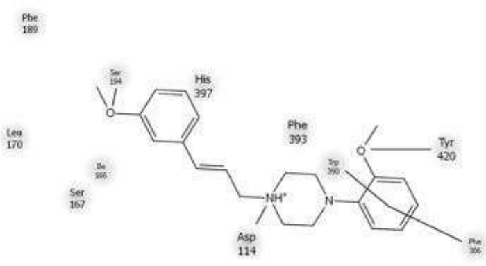
Docking schematics results of ligands 20 (upper left), 21 (upper right), 23 (lower left) and 16 (lower right)
