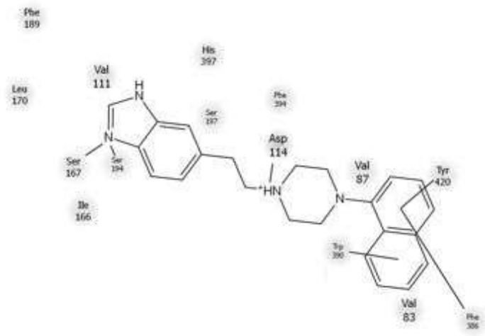
Docking schematics results of ligands 20 (upper left), 21 (upper right), 23 (lower left) and 16 (lower right)
