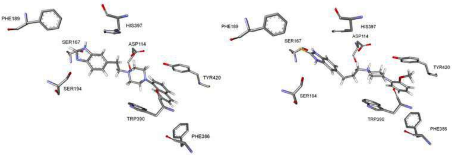
Docking results of ligands 16 (left) and 20 (right)
