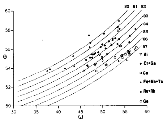
Fig. 2. X-ray structures of [M(\text{ox})_3]^{3-} ions on the \theta - \omega plot showing that most of the structures approximately follow the relationship \cos(\omega/2) = \cos(\alpha/2)/\sin(\theta) , and that metal ions of similar ionic radii have approximately similar \alpha angles. The dotted lines correspond to constant values of \alpha , indicated in the upper right corner of the graph. All data extracted from CSD 17 are shown. 18
