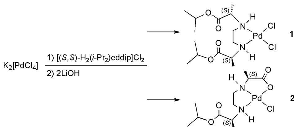
Scheme 1. Reaction of K_2[PdCl_4] with [( S,S )- H_2(i\text{-Pr})_2\text{eddip} ] Cl_2 .
