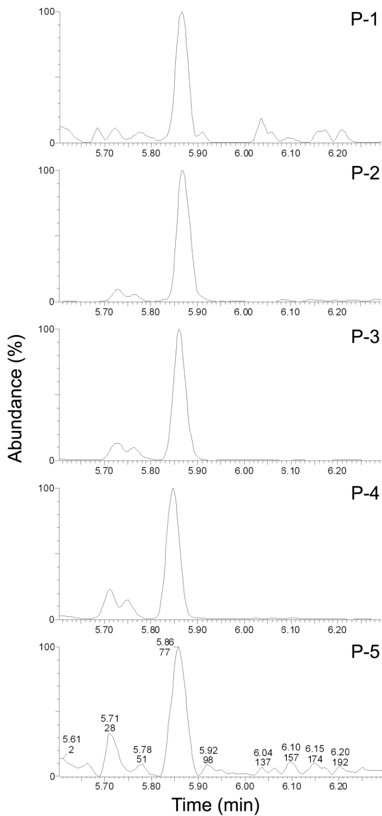
Figure 1. Mass chromatograms of the molecular ion m/z 499 of PFOS (samples P-1, P-2, P-3, P-4 and P-5)
