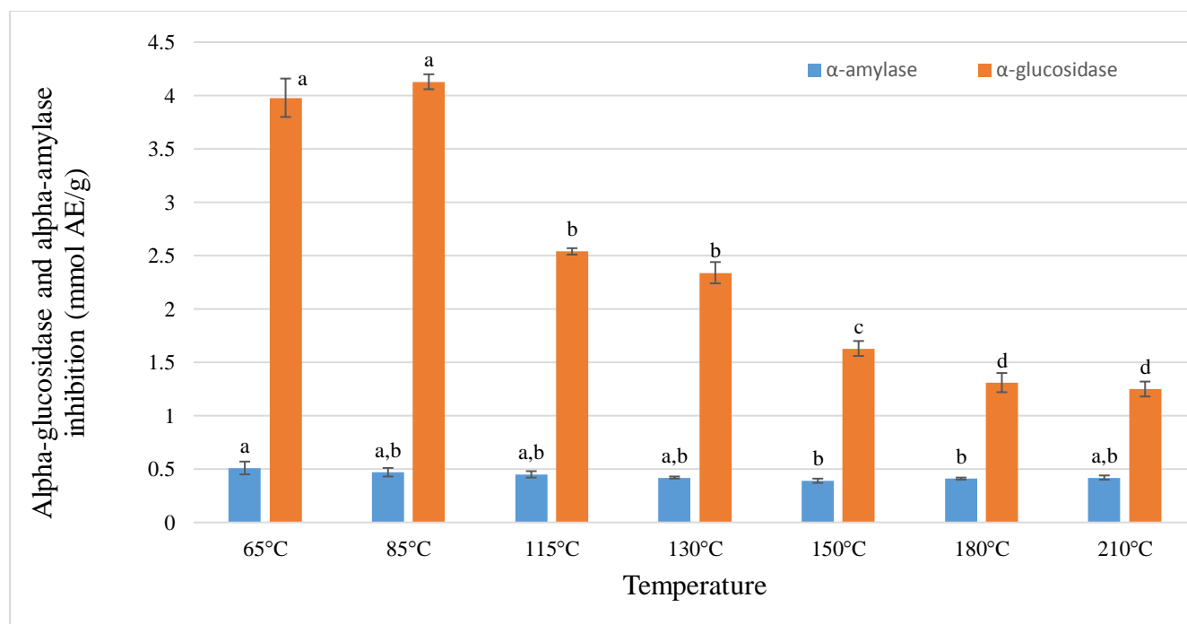
Figure 1. The activity of chamomile extracts obtained at different temperatures against \alpha -glucosidase and \alpha -amylase inhibition; Significant differences among the samples obtained at different temperatures are indicated by different letters ( P < 0.05 ). Error bars represent standard error of the mean for 3 replicates.
