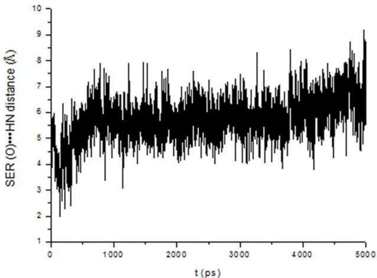
Change of distance between SER 197 oxygen and NH hydrogen of ligand during production phase
