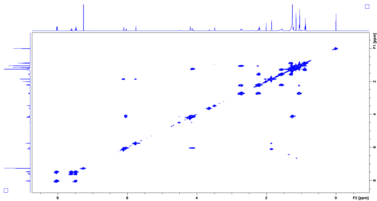
NOESY benzoyl Ingenol-laurate (1),
