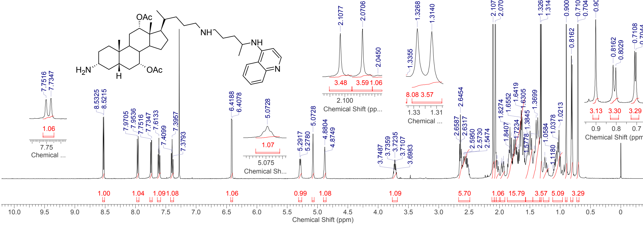
(3a,5b,7a,12a)-3-Amino-24-[[4-(quinolin-4-ylamino)pentyl]amino]cholane-7,12-diyl diacetate (17)
