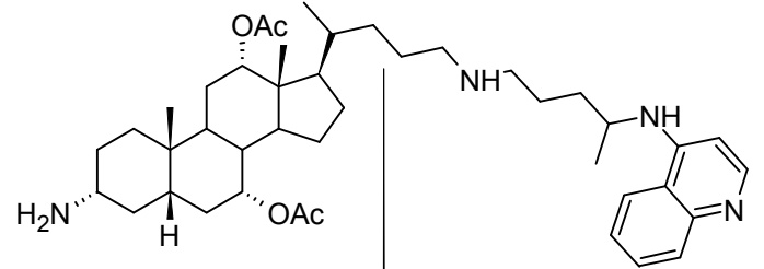
(3a,5b,7a,12a)-3-Amino-24-[[4-(quinolin-4-ylamino)pentyl]amino]cholane-7,12-diyl diacetate (17)
