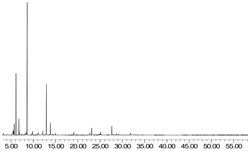
Figure 3S: GC of the essential oil from Tanacetum macrophyllum isolated using Static headspace apparatus
