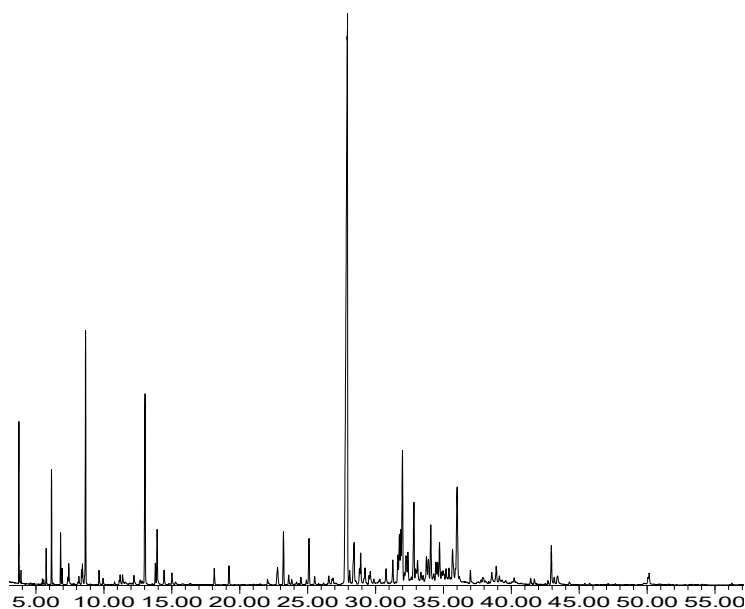
Figure 1S: GC of the essential oil from Tanacetum macrophyllum isolated using Clevenger-type apparatus
