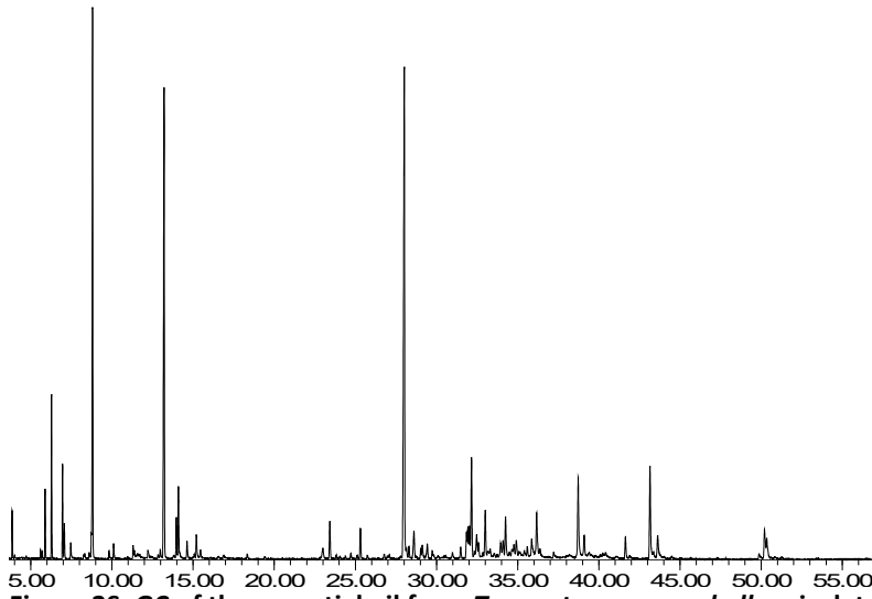
Figure 2S: GC of the essential oil from Tanacetum macrophyllum isolated using Likers Nickerson apparatus
