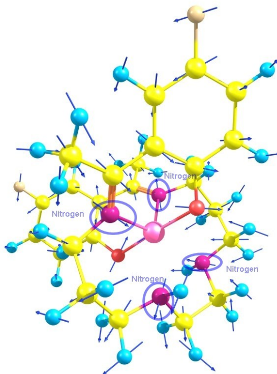
Fig. S7.- Graphical representation of the vibrational mode with \hbar\omega_7 = 78.6 \text{ cm}^{-1} showing a b 1 -like distortion where two nitrogen ions move inwards towards Mn and two move outwards from Mn.
