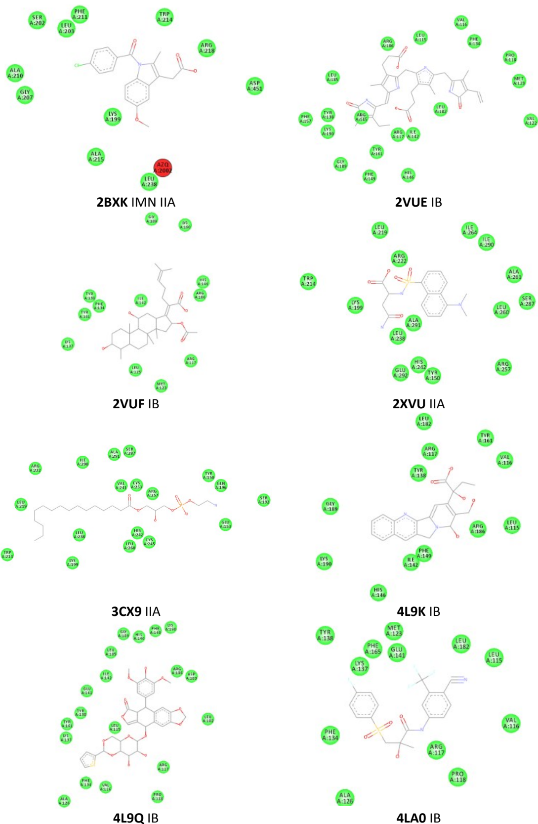
Figure S1 Amino acid residues within 3.5Å from the ligand/drug binding site (IIA or IB) for ligands/drugs from selected HSA crystal structures.
