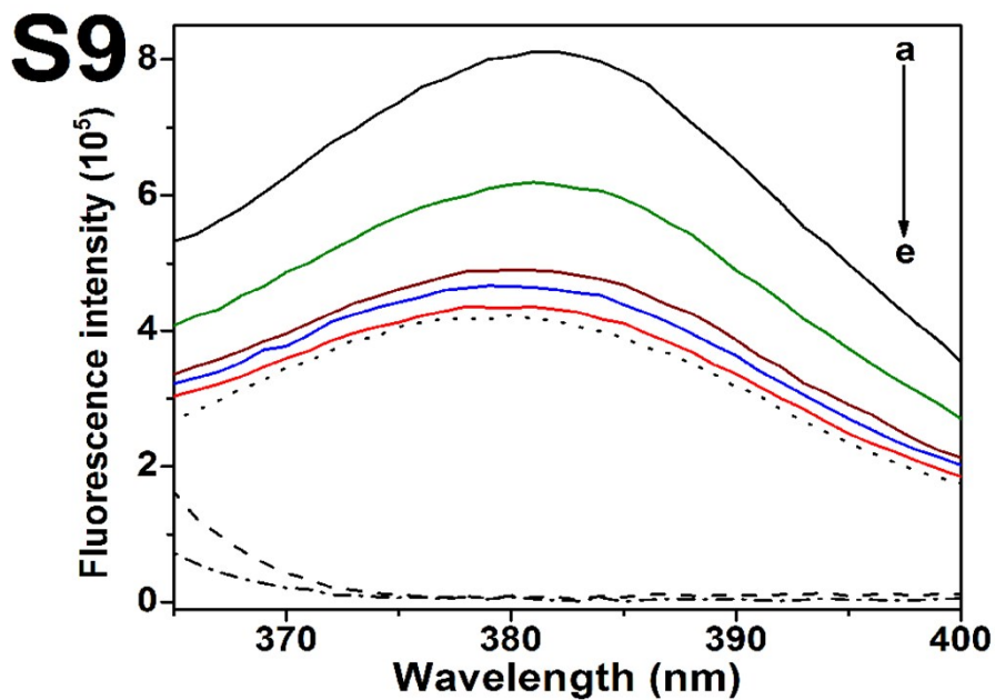
Figure S9 Quenching of HSA-warfarin complex (0.25 μM both) by bilirubin (0, 0.125, 0.25, 0.375, and 0.5, for curves a to e, respectively) using synchronous fluorescence spectroscopy, \Delta\lambda 64 nm. Dash line curve: 0.25 μM HSA. Dot line curve: 0.25 μM warfarin. Dash-dot line curve represents 0.25 μM HSA in presence of 0.5 μM bilirubin.
