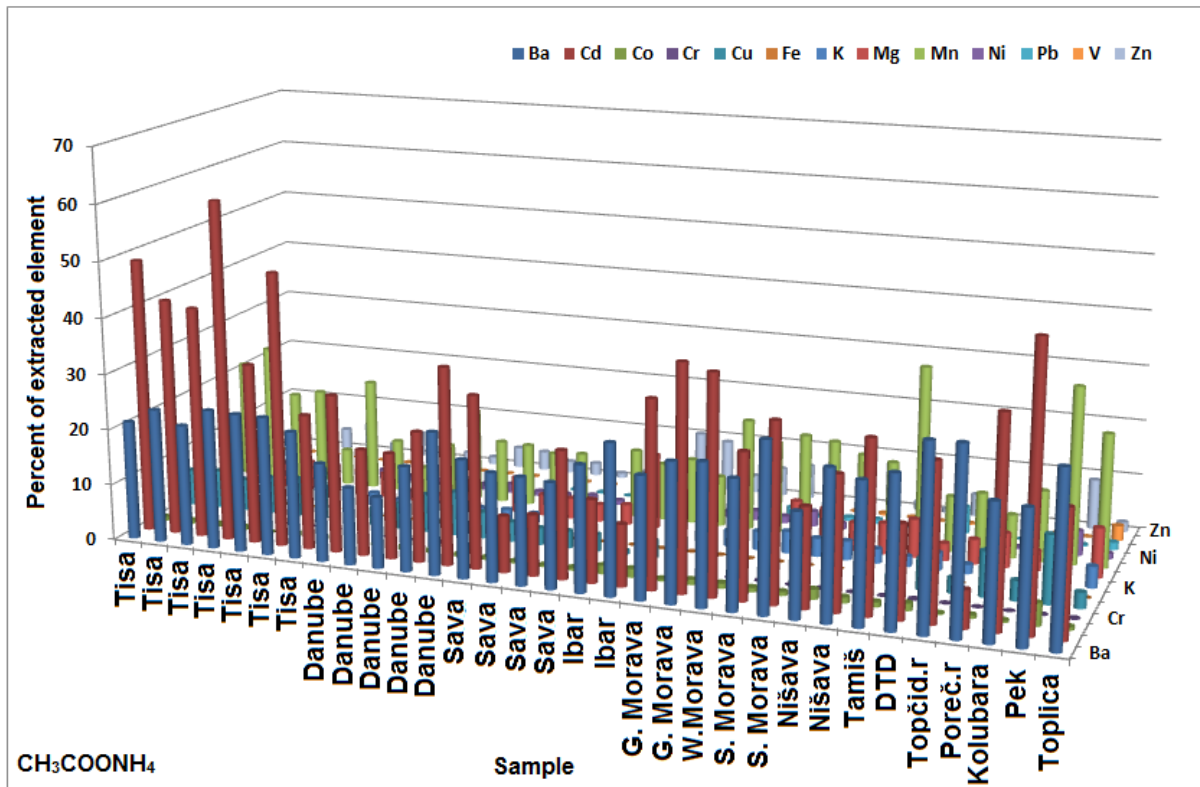
Suppl. Fig. 4. Percent of extracted element (extraction with CH 3 COONH 4 )
