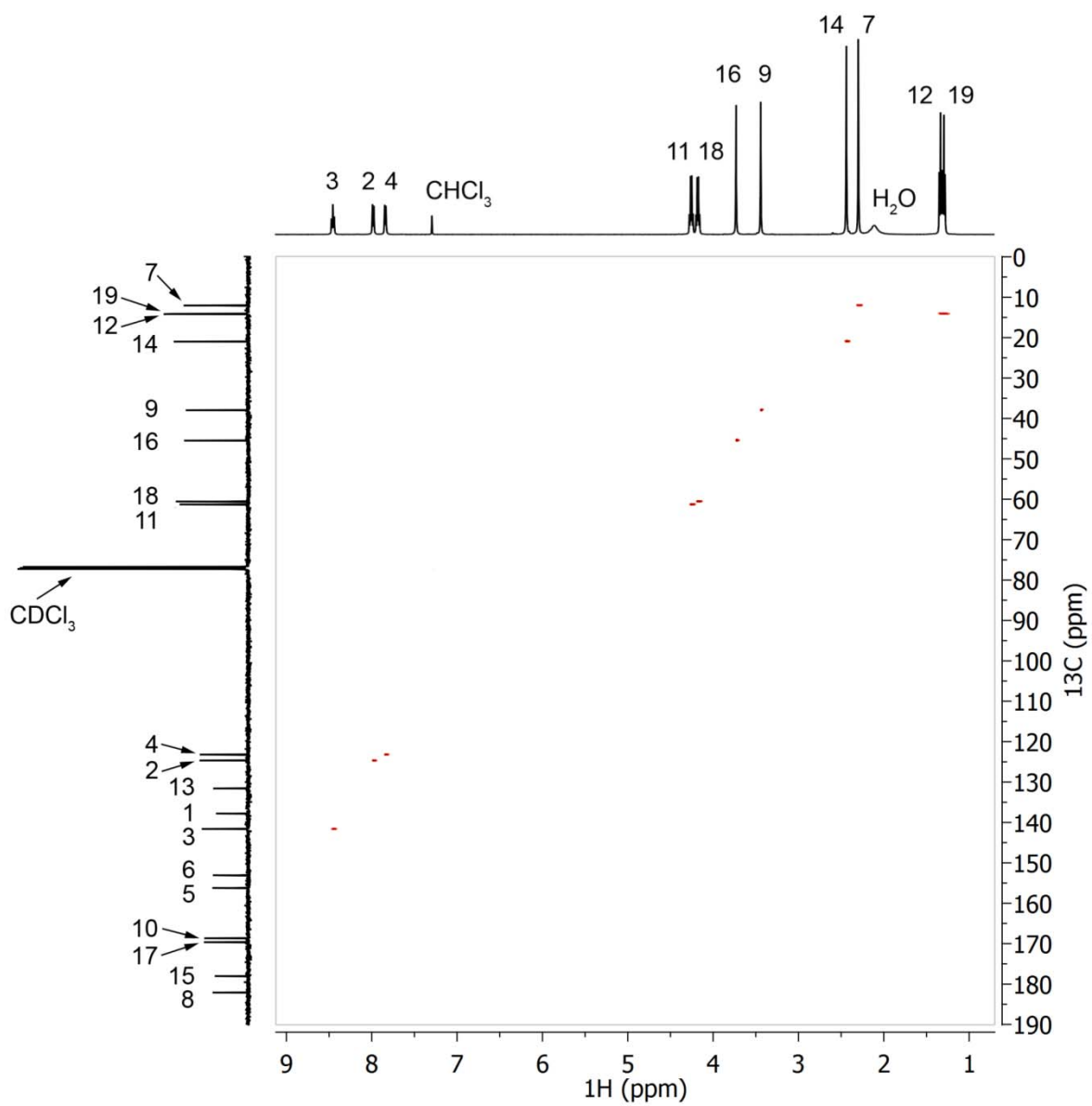
Figure S7. ^1\text{H} - ^{13}\text{C} HSQC NMR spectrum of 1 in \text{CDCl}_3 .
