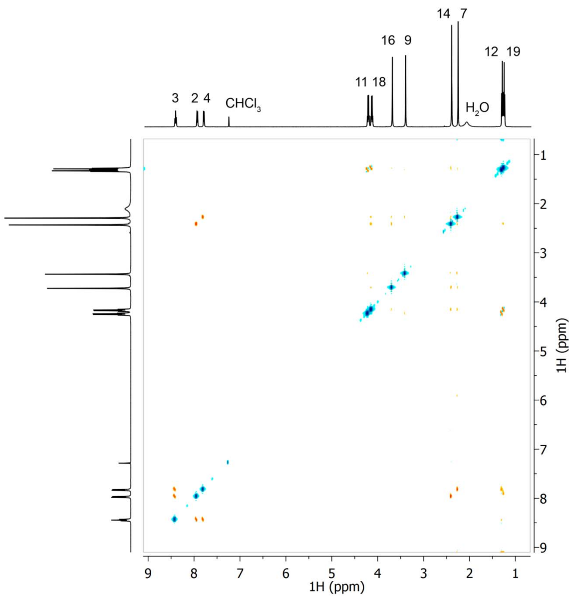
Figure S6. ROESY spectrum of 1 in CDCl 3 .
