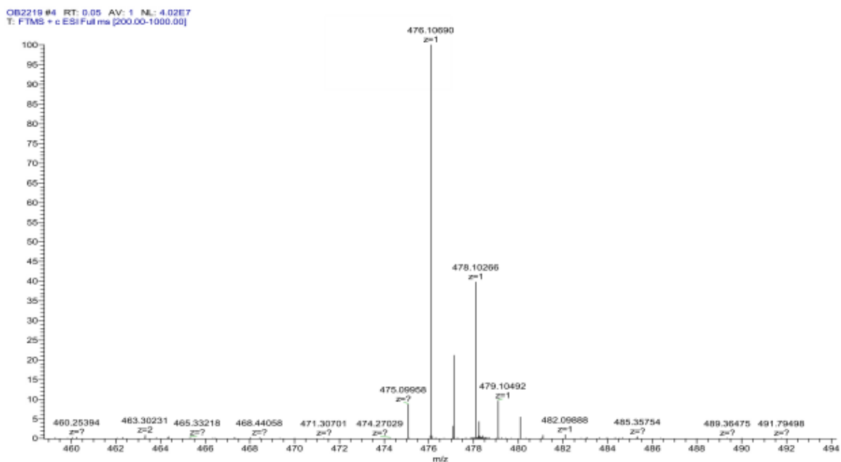
Figure S1. Mass spectrum of 1 in acetonitrile.
