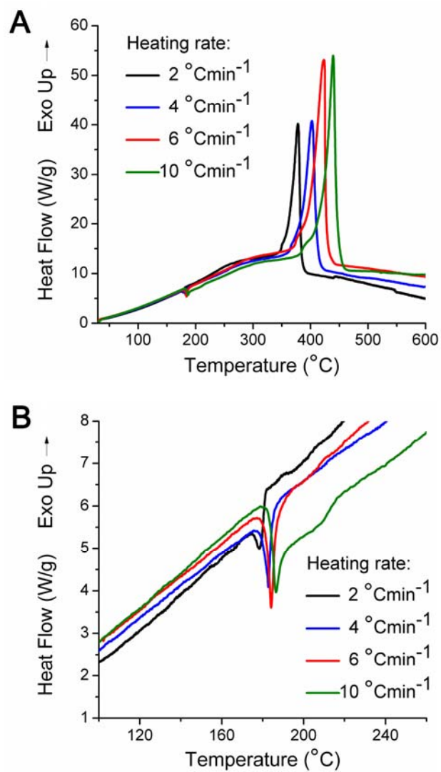
Figure 13. DSC curves in air with subtracted baselines at different heating rates (A), with enhanced region of the first degradation peak (B).
