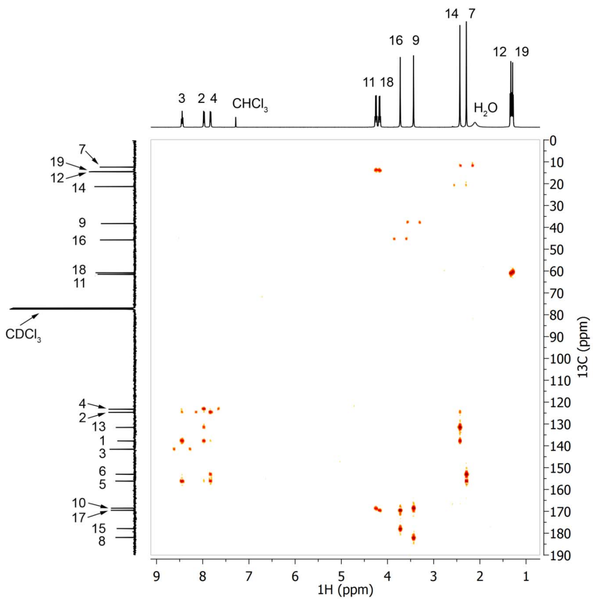
Figure S8. ^1\text{H} - ^{13}\text{C} HMBC NMR spectrum of 1 in \text{CDCl}_3 .
