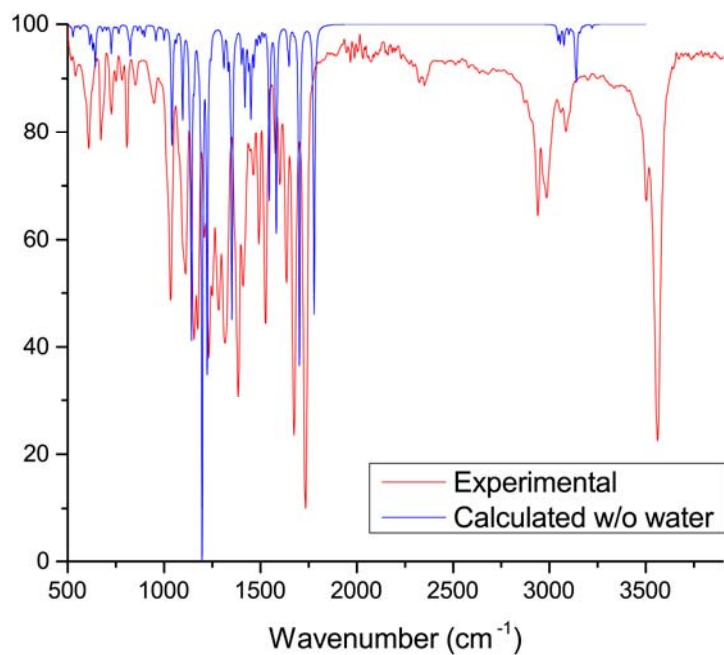
Figure S11. Comparison of experimental IR spectrum and calculated IR spectrum for the structure with coordination of the carbonylic oxygen of the hydrazonic arm.
