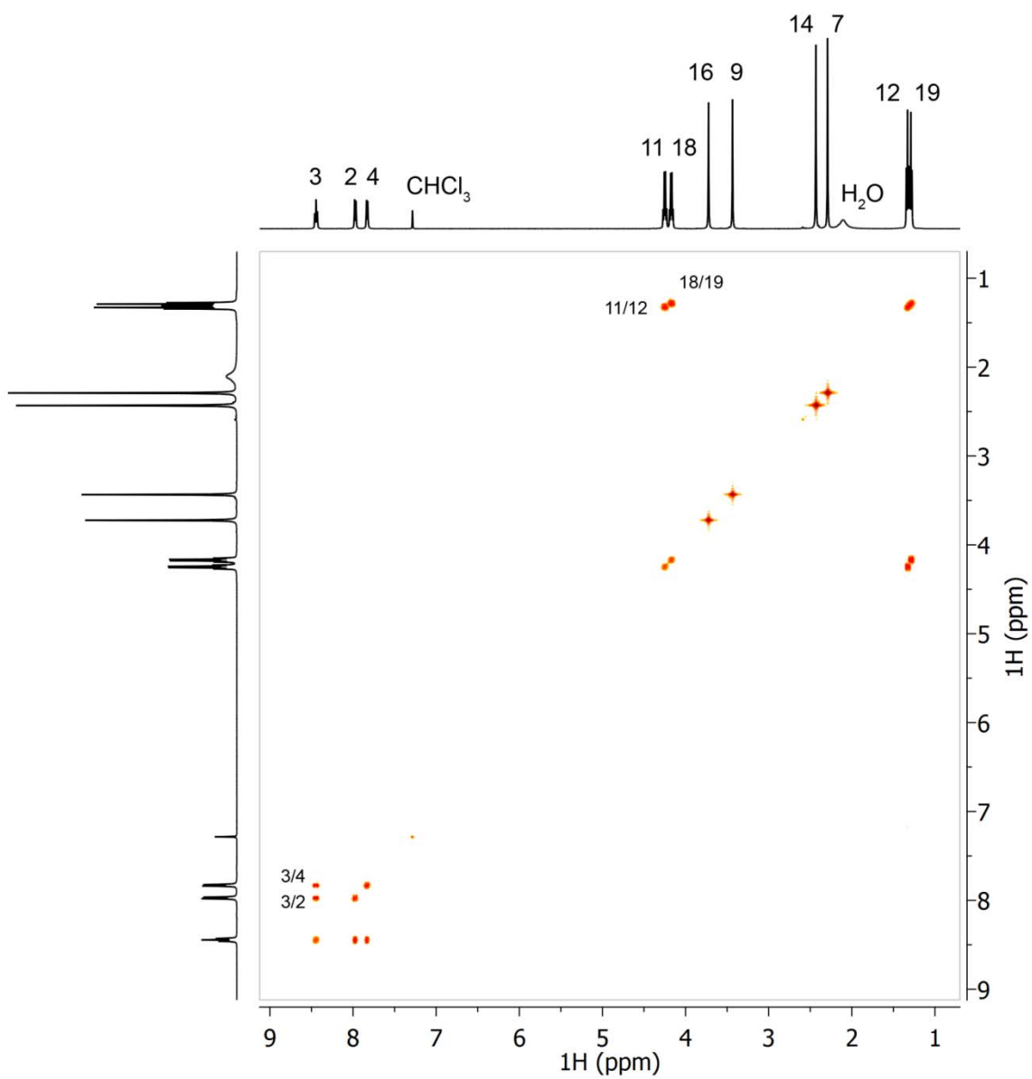
Figure S4. COSY spectrum of 1 in CDCl 3 .
