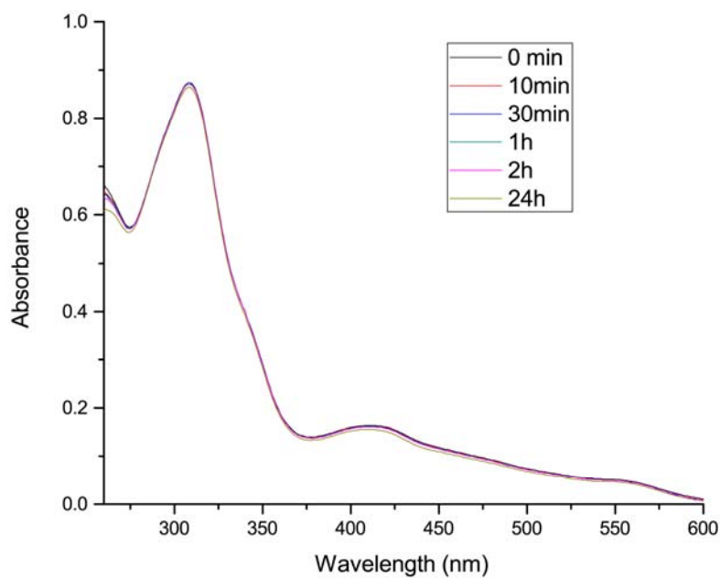
Figure S12. UV-VIS spectra of 1 in DMSO over 24 hour period.
