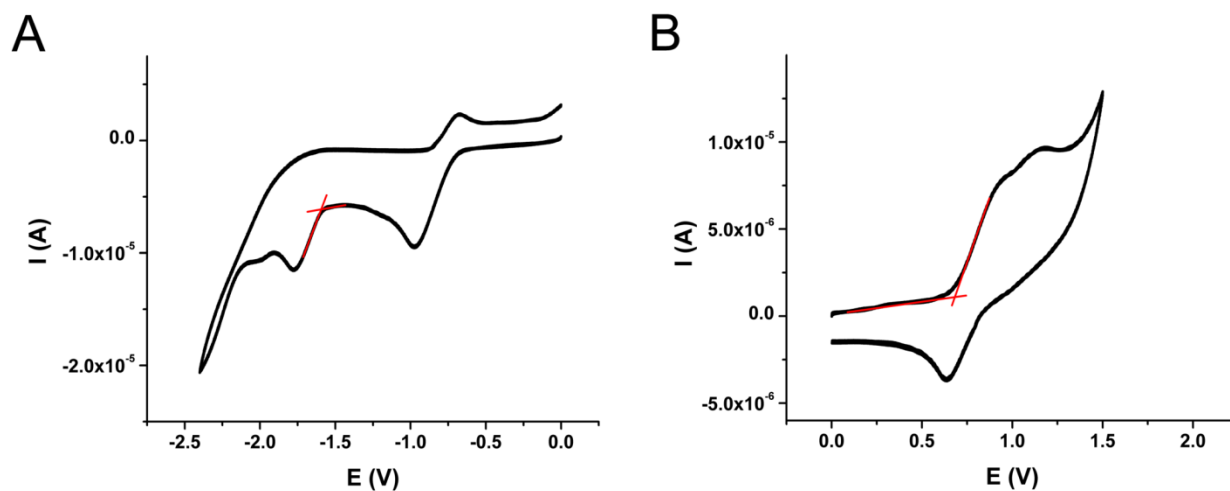
Figure S9. Cyclic voltammograms of 1 in anhydrous DMSO containing 0.10 M [n\text{-Bu}_4\text{N}][\text{PF}_6] at a scan rate of 100 \text{ mVs}^{-1} using a glassy carbon working electrode in the potential range from -2.5 to 0.0 V (A) and from 0.0 to +1.5 V (B).
