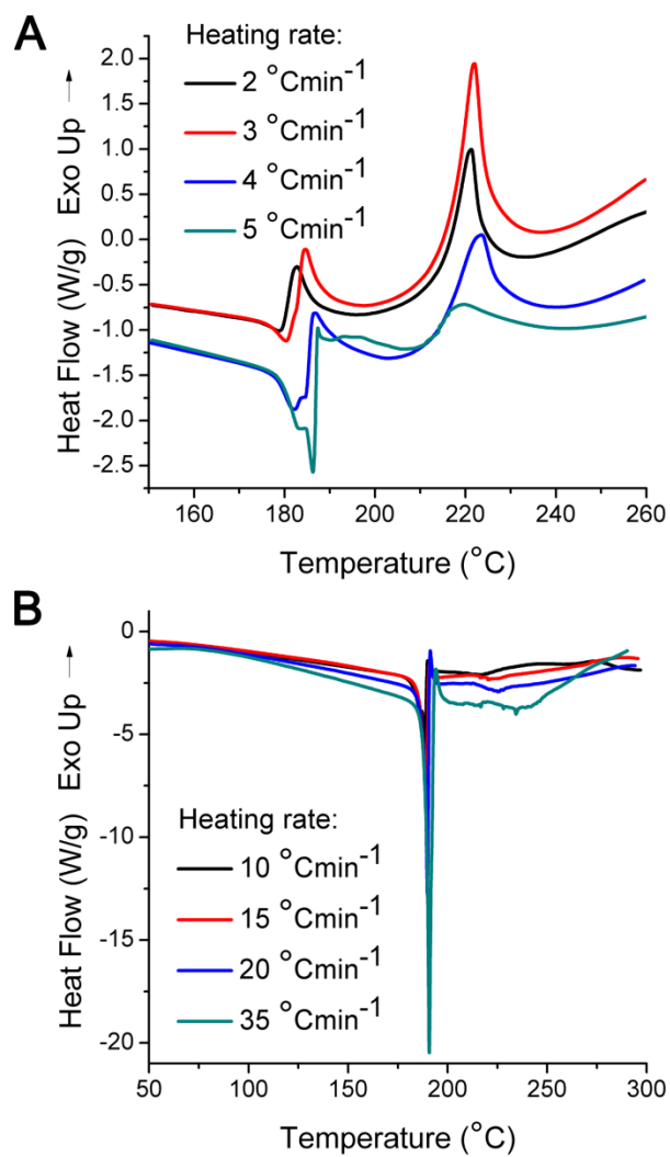
Figure S14. DSC recorded in nitrogen at lower (A) and higher (B) heating rates.
